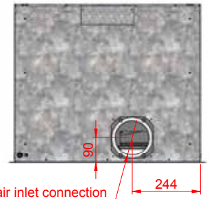
REAR
